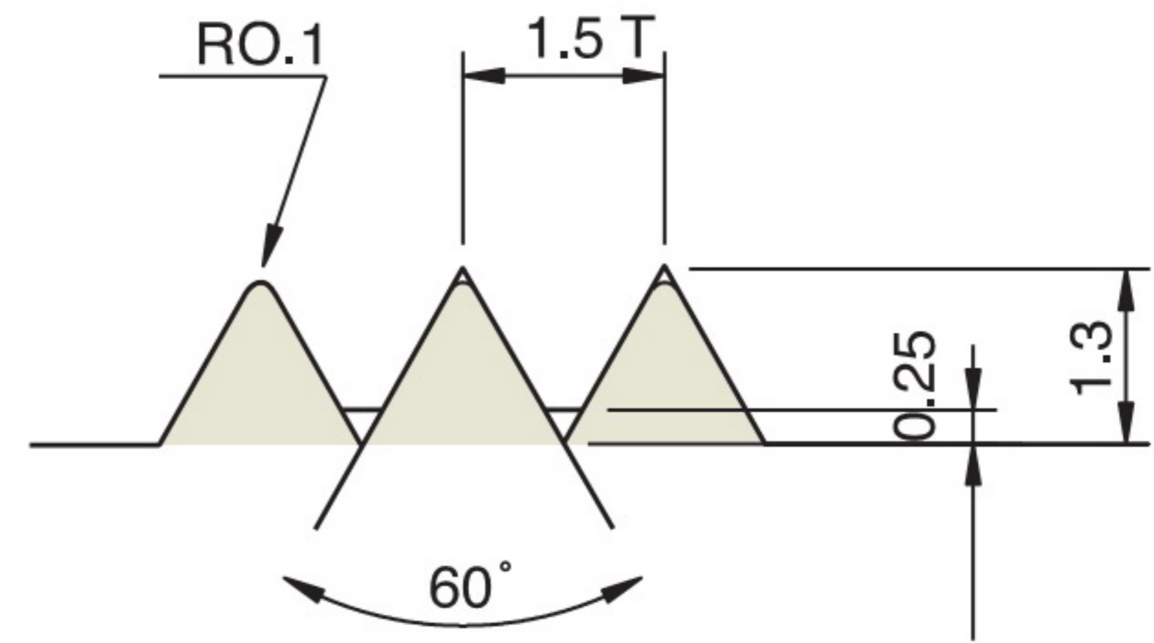
排齒詳圖 Drawing of Serration
